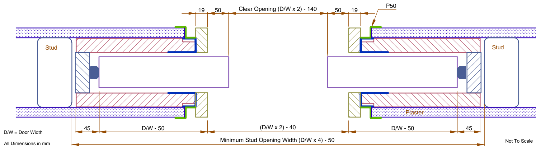
Double Architectural P50 Shadow Line 19mm Reveal (Flush Pull)
